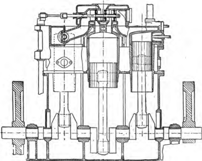
FIG. 138.—Crossley Three-Cylinder Compound Gas Engine. The two end cylinders are high pressure; the central one, low pressure. The exhaust from the two high-pressure cylinders is admitted, alternately, to the low-pressure cylinder by the piston valve, operated by the crank and rotating shaft shown at the left. The exhaust from the low-pressure cylinder passes upward through the port at its top.
